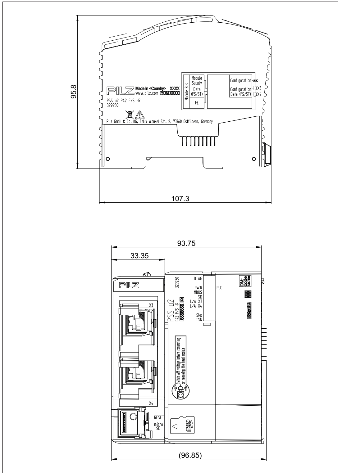
Fig.: Dimensions of head module PSS u2 P42 F/S -R (without main voltage supply module)
