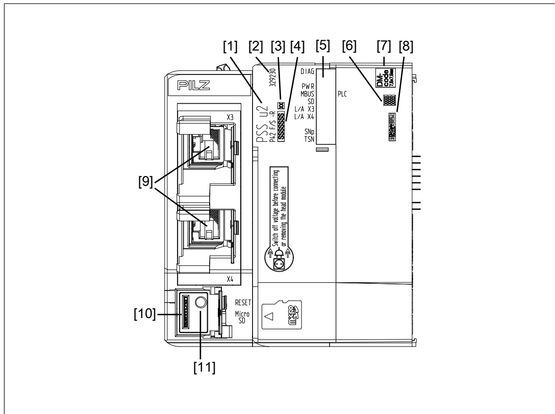
Front view of head modules with an RJ45 female connector
