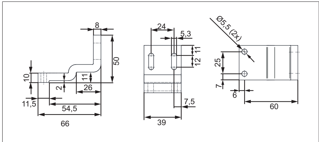
Fig.: Mounting bracket for swing gate (see Accessories [63])
