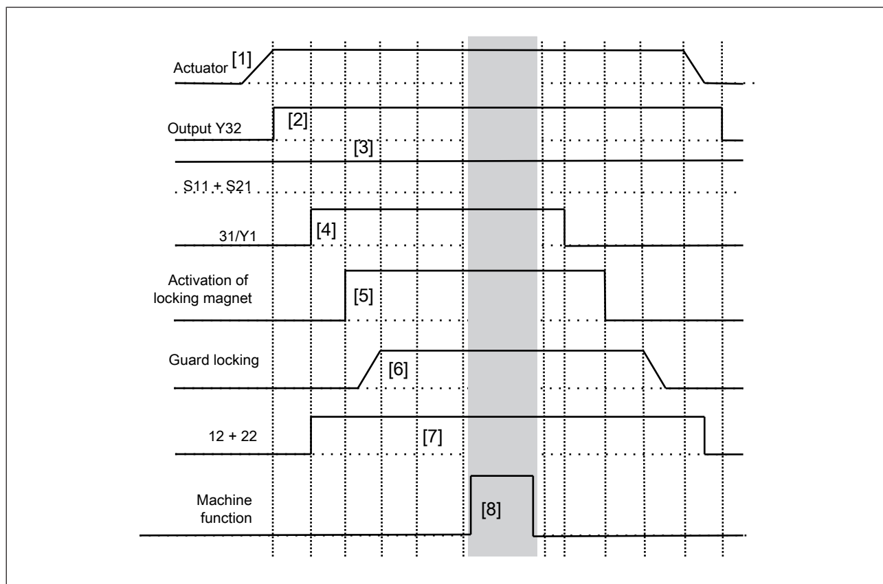
Fig.: Guard locking is controlled via 31
