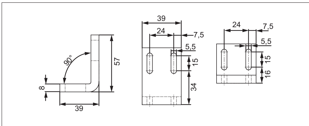
Fig.: Mounting bracket for sliding gate (see Accessories [63])
