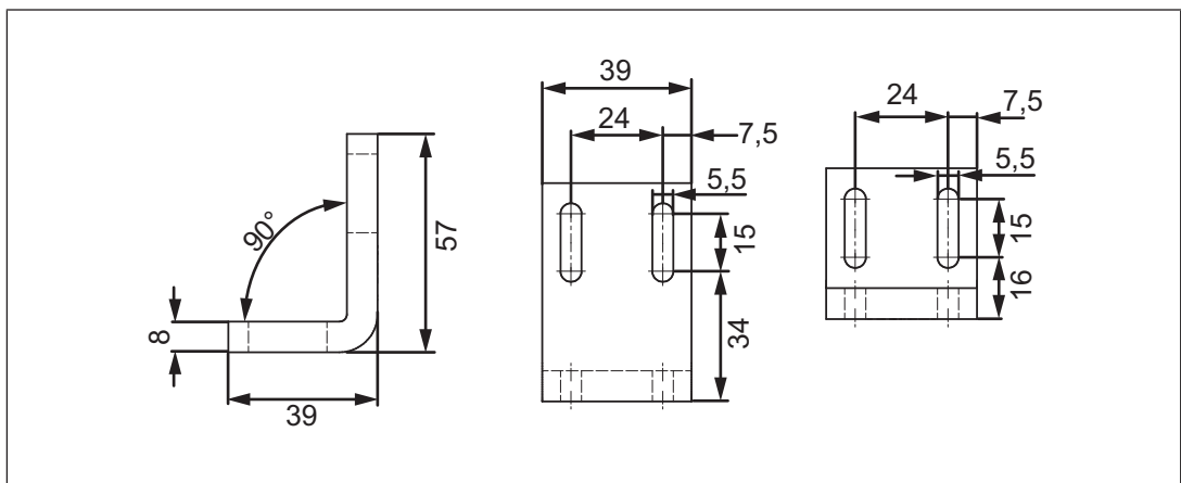
Fig.: Actuator PSEN sl2-L-VA-actuator - front view, side view, rear view
