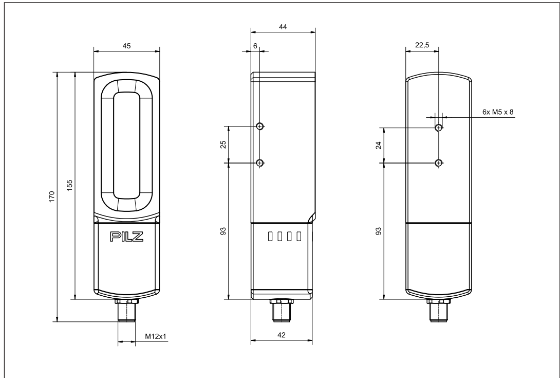
Fig.: Safety switch - front view, side view, rear view
