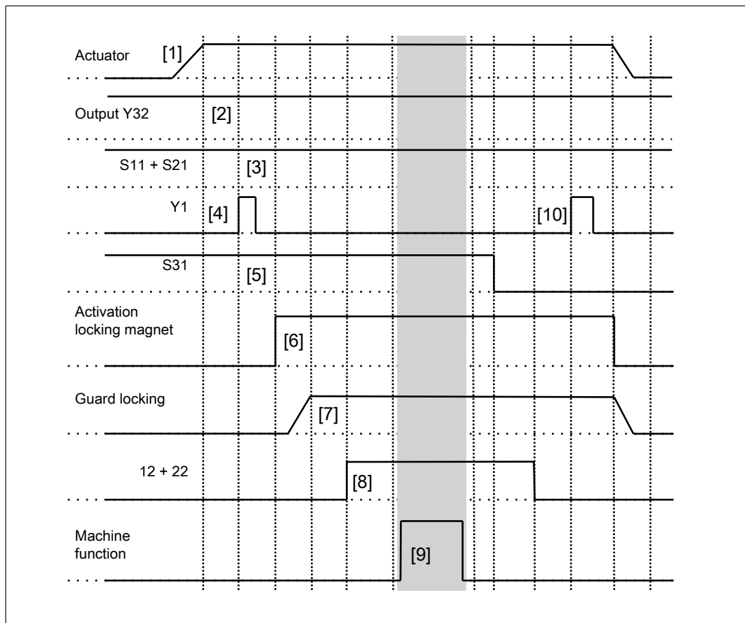
Fig.: Active use of Safety Device Diagnostics
