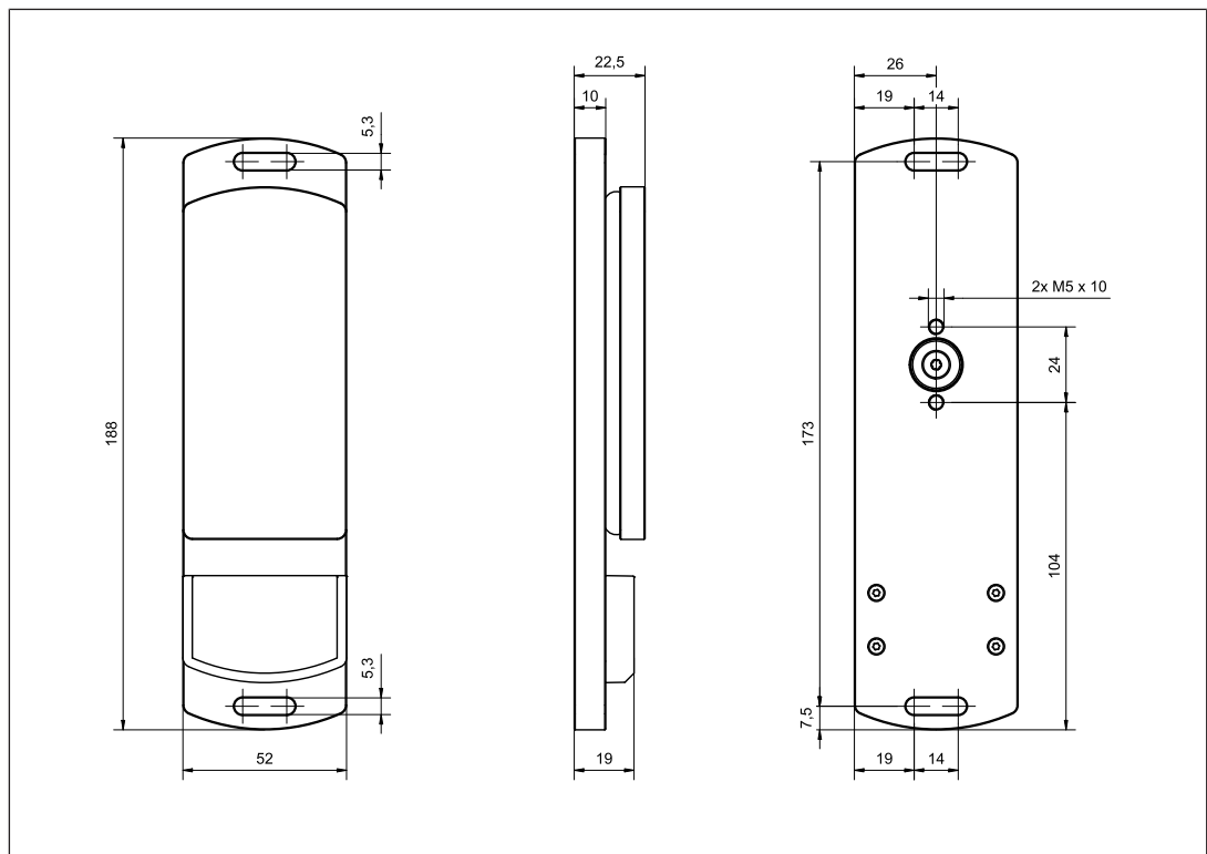
Fig.: Actuator PSEN sl2-L-AL-actuator - front view, side view, rear view
