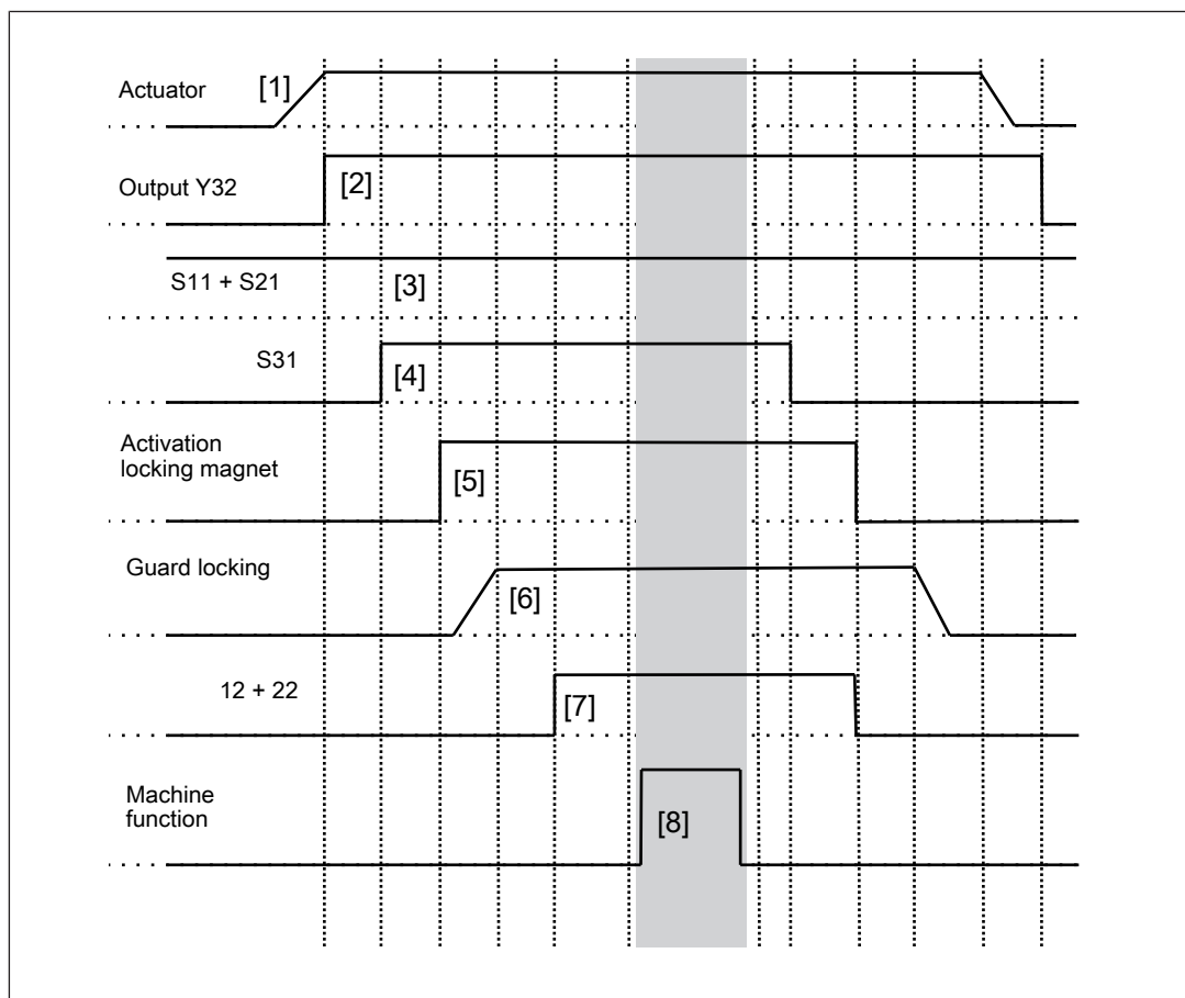
Fig.: Guard locking is controlled via S31
