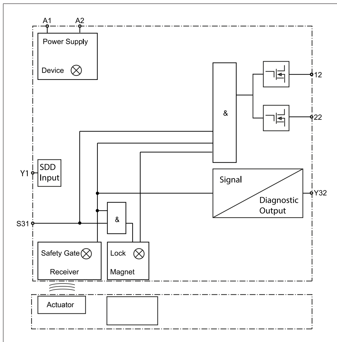
Block diagram
