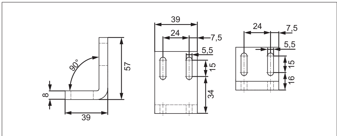
Fig.: Mounting bracket for sliding gate (see Accessories [49])
