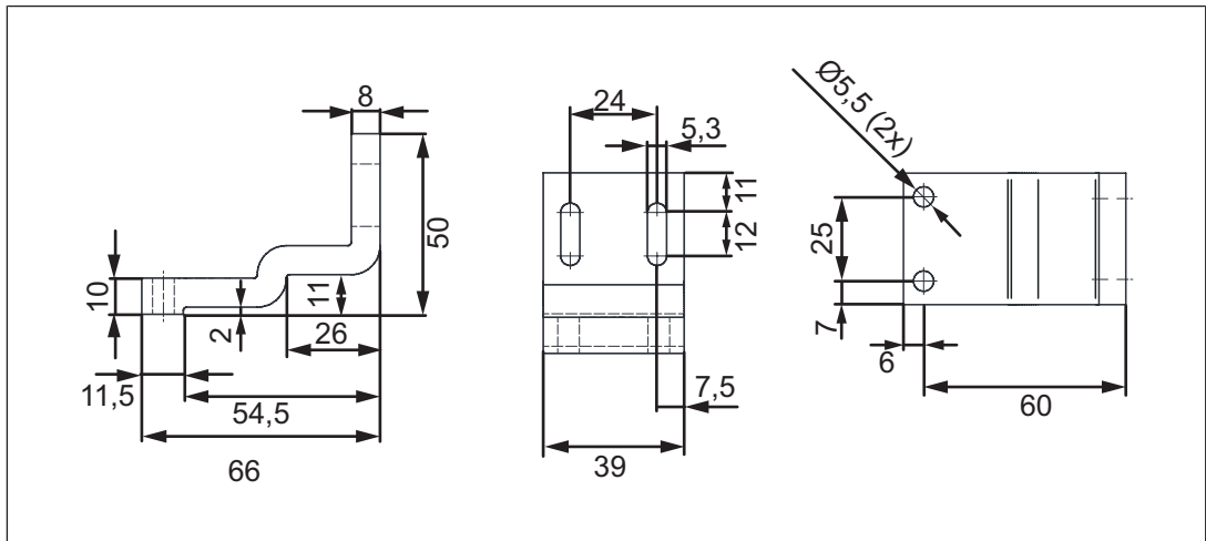
Fig.: Mounting bracket for swing gate (see Accessories [49])
