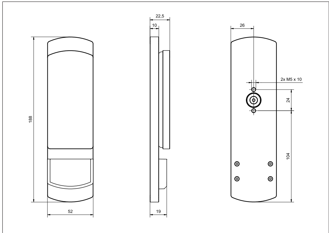
Fig.: Actuator PSEN sl2-L-VA-actuator - front view, side view, rear view
