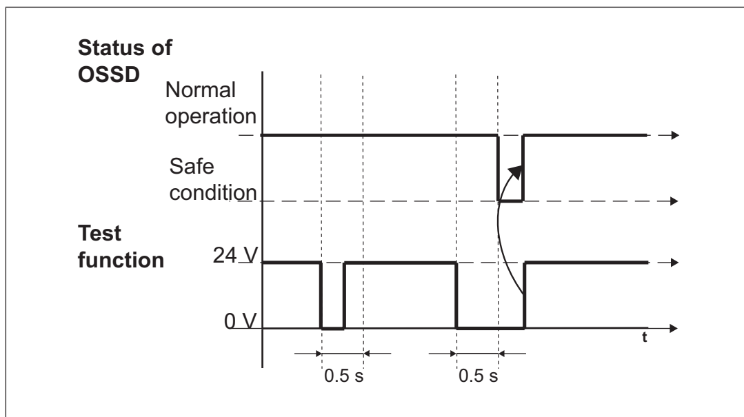
Fig.: Timing diagram for test function
