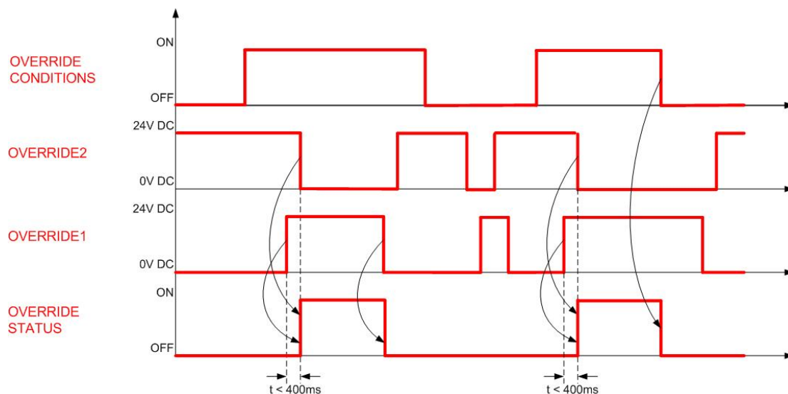
Fig. 47 – Override timings (activated by level)
