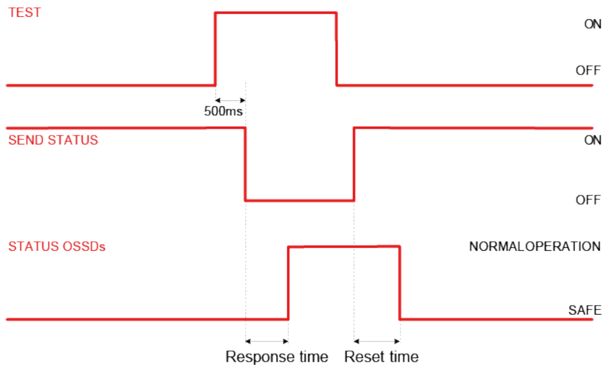
Fig. 34 – Test timings
