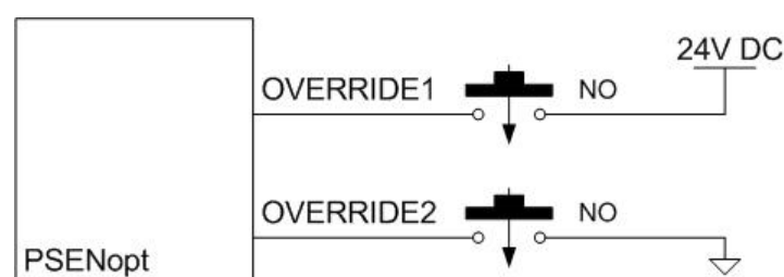
Fig. 46 – Override connection
