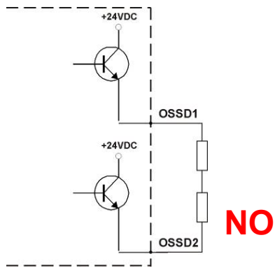
Fig. 24 – Incorrect OSSD signal load connection (II)
