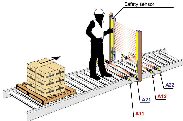
Fig. 40 – Typical muting application
