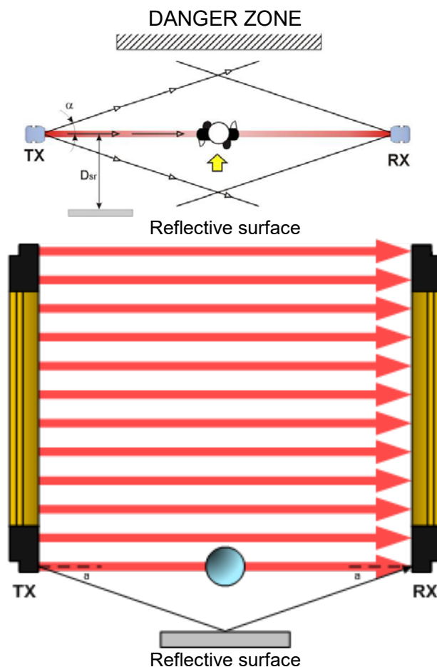
Fig. 9 Minimum distance from reflective surfaces
