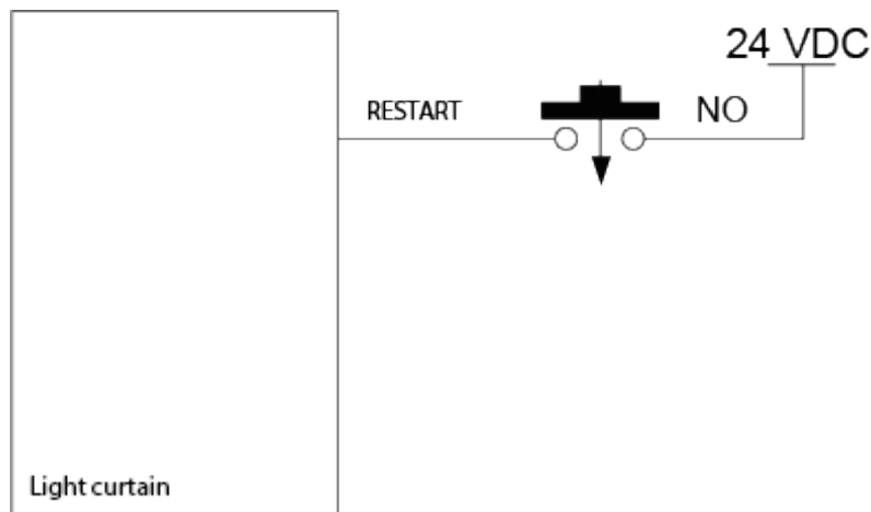
Fig. 33 – Restart connection (manual)
