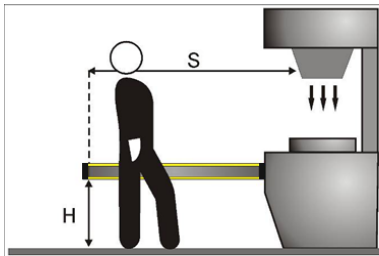
Fig. 4 – Safety distance (horizontal)
