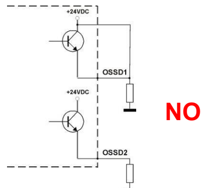
Fig. 23 – Incorrect OSSD signal load connection (I)
