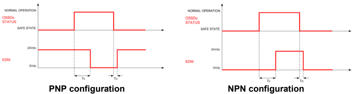
Fig. 36 – EDM timings
