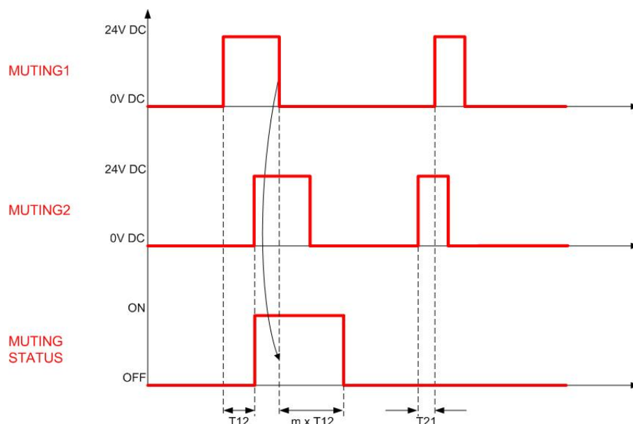
Fig. 43 – L-muting timings
