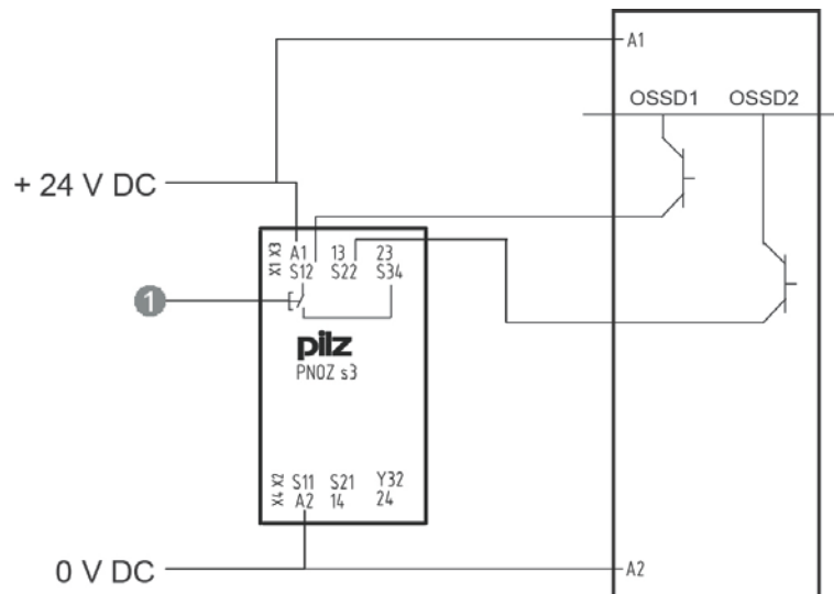
Fig. 21 – Connection to safety relay – manual start
