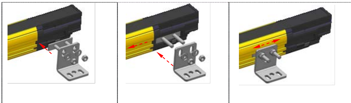
Fig. 17 – Procedure with fixed mounting brackets
