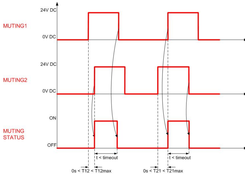
Fig. 41 – T muting timings
