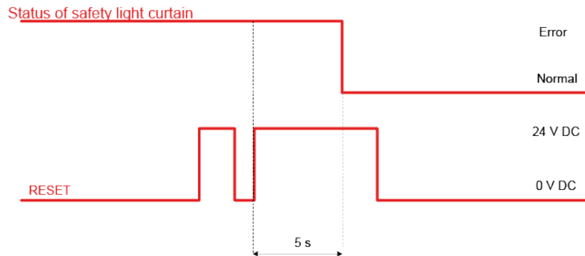
Fig. 35 – Reset timings
