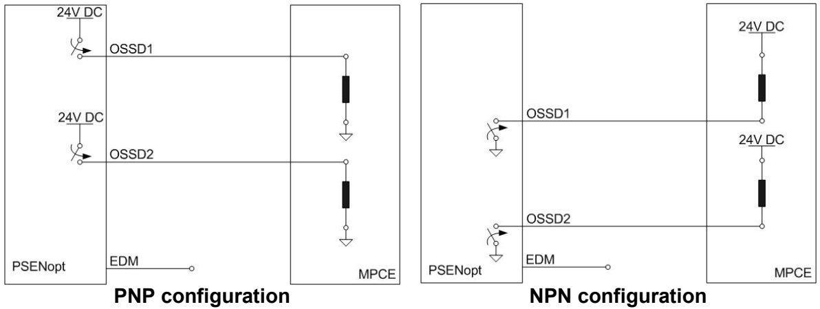
Fig. 37 – EDM connections
