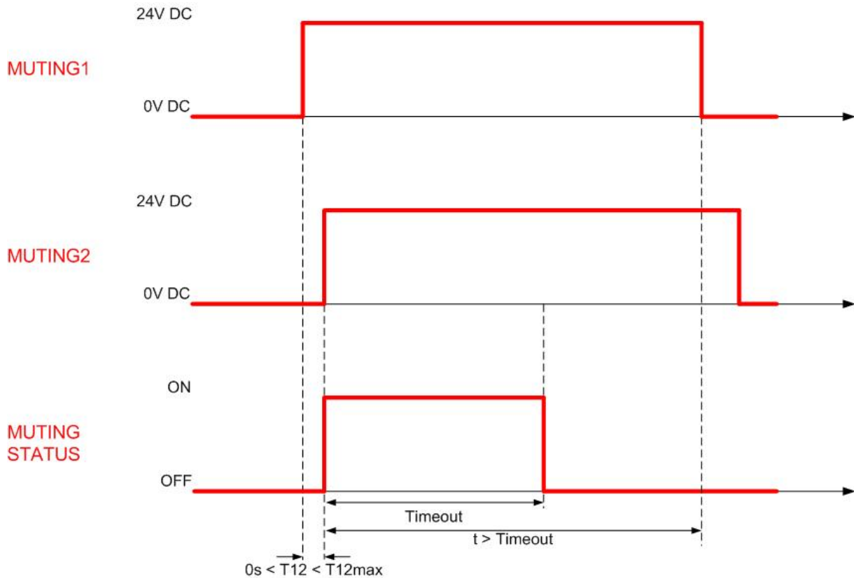
Fig. 45 – Muting timeout
