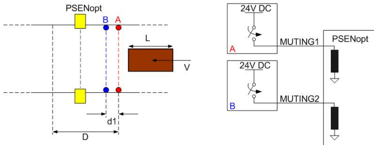
Fig. 44 – L-Muting connection
