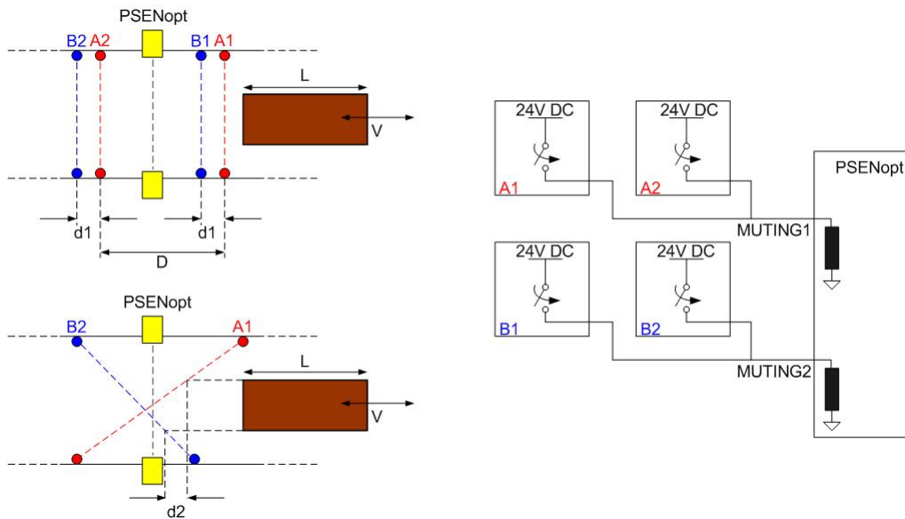
Fig. 42 – T-Muting connection
