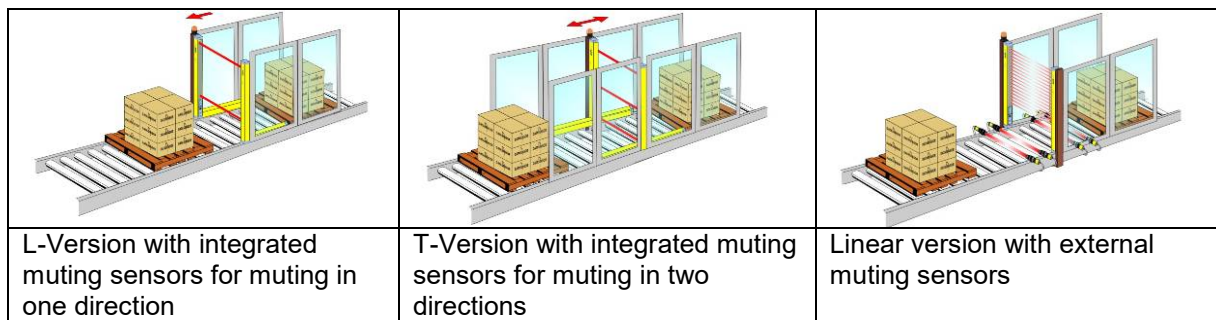
Fig. 39 – Application examples for the muting function
