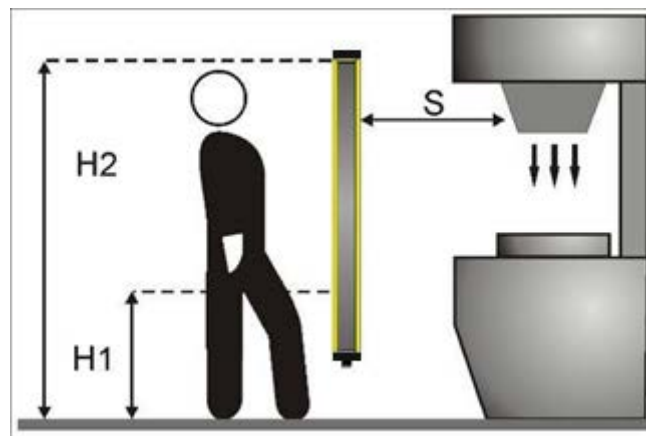
Fig. 3 – Safety distance (vertical)
