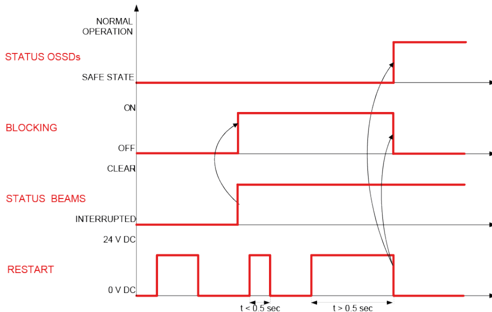
Fig. 32 – Restart timings (manual)
