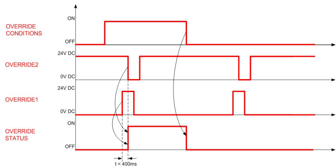
Fig. 48 – Override timings (activated by edge)
