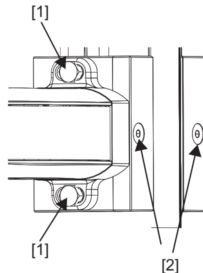
[1] Hexagonal screws for attaching the mounting profile to the safety light grid
