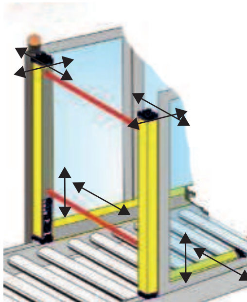
The yellow LEDs High Align [3] and Low Align [4] indicate the status of the alignment.
