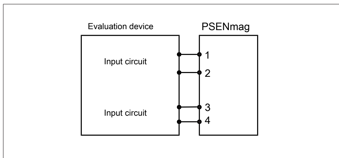
Fig.: Dual-channel connection PSEN ma1.4p-50 to the input circuits of an evaluation device
