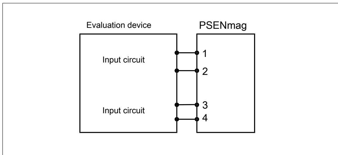
Fig.: Dual-channel connection PSEN 1.2p-20 to the input circuits of an evaluation device
