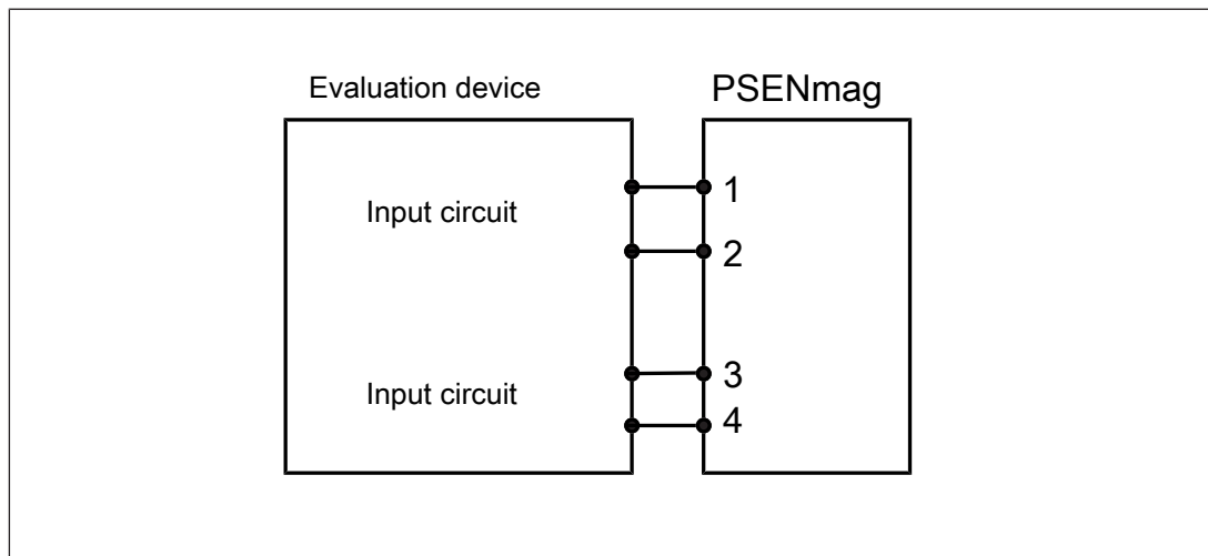
Fig.: Dual-channel connection PSEN 1.1p-20 to the input circuits of an evaluation device
