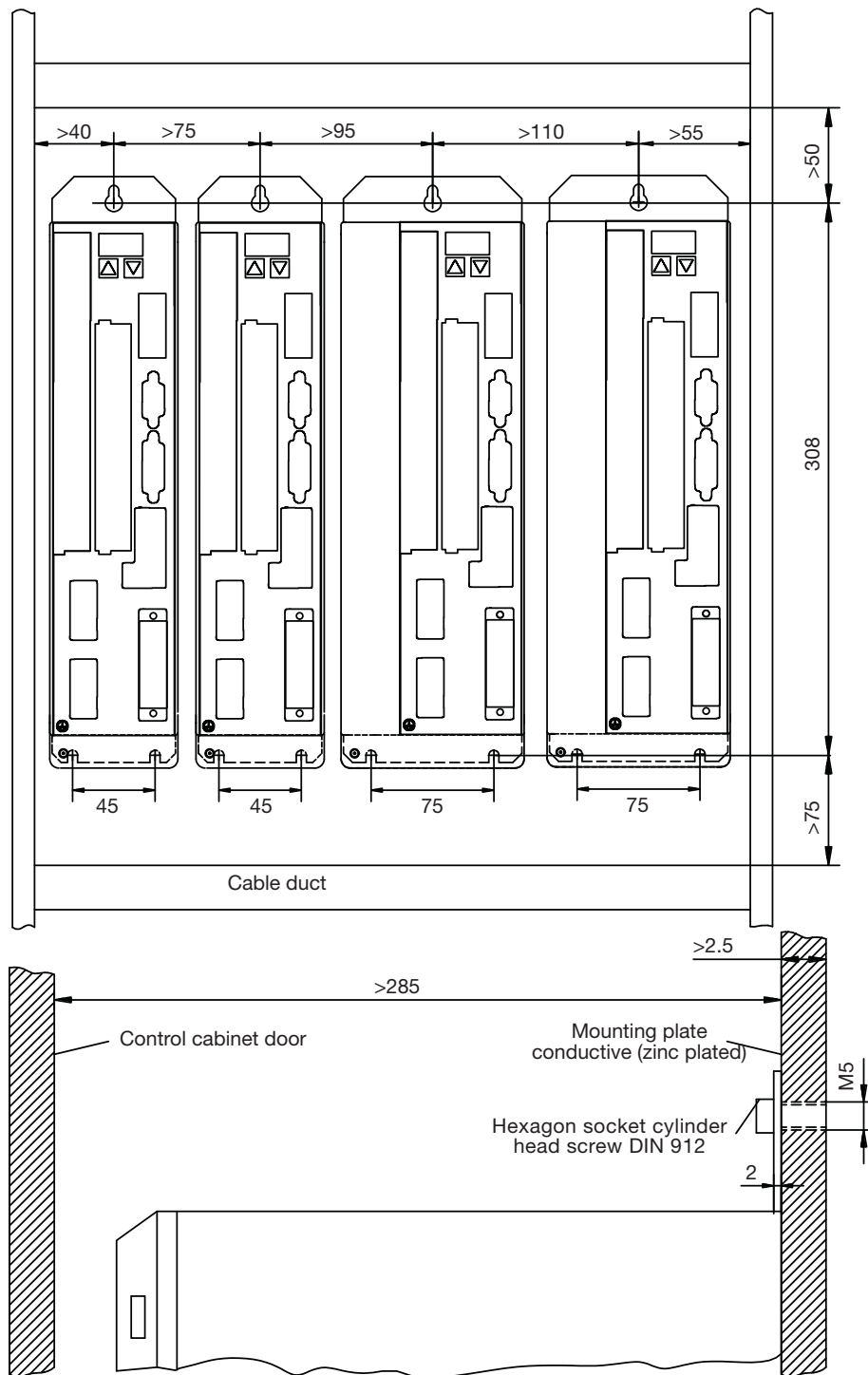
Fig.: Installing the servo amplifier in a control cabinet
