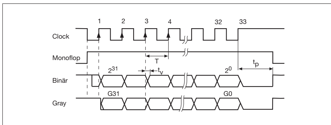
Fig.: Timing diagram in gray and binary code
