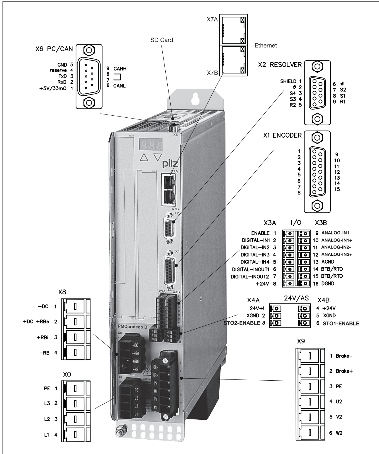
Fig.: Connector description for PMcprotego D
