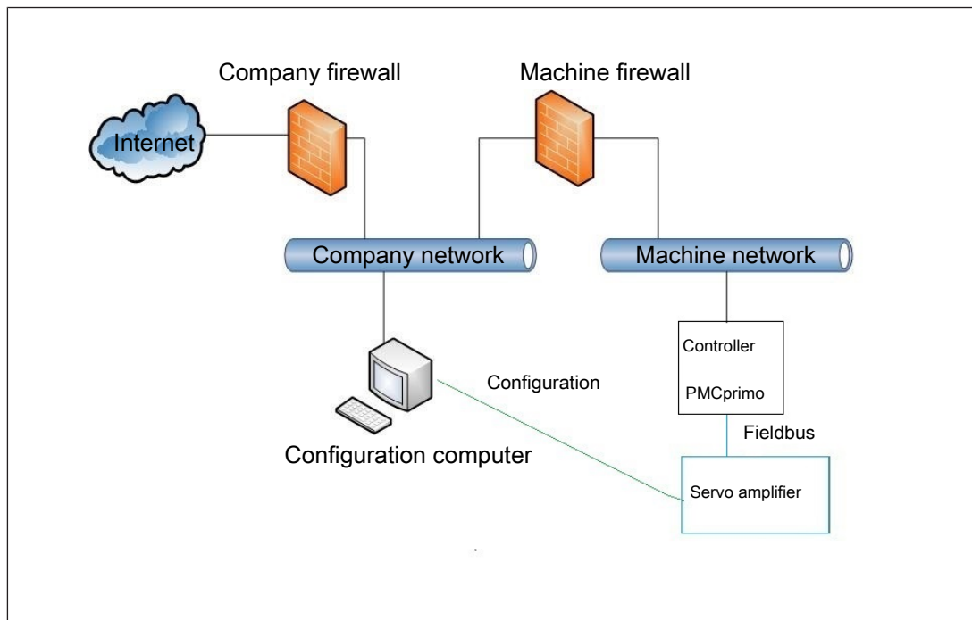
Fig.: Network topology PMCprotego D
