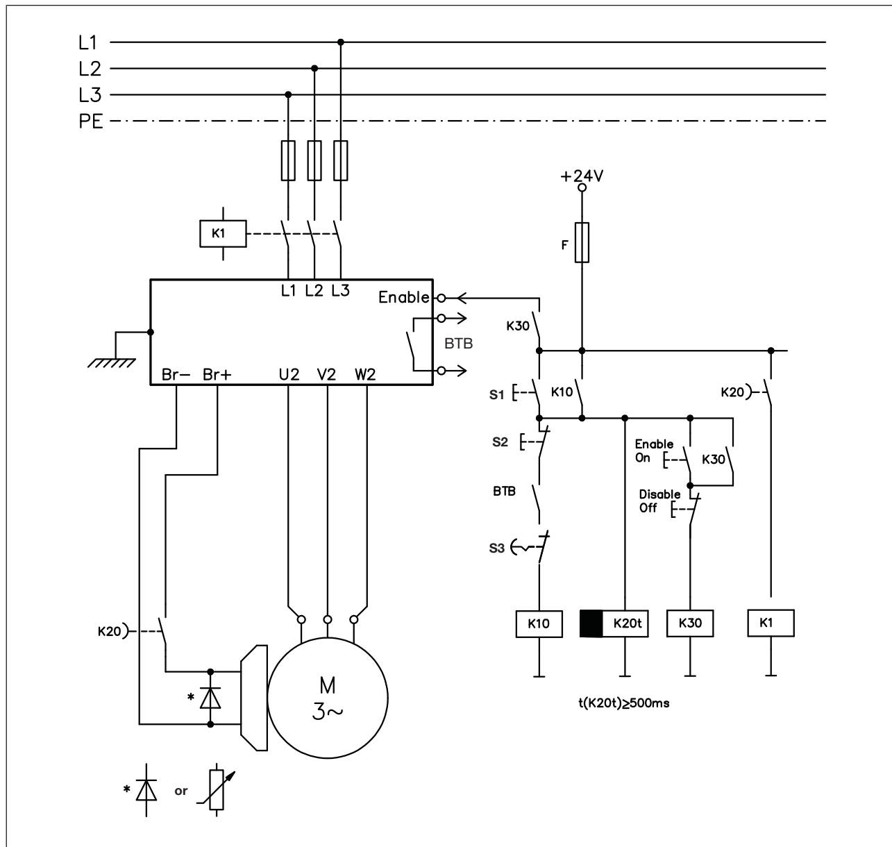
Fig.: Stop category 2
