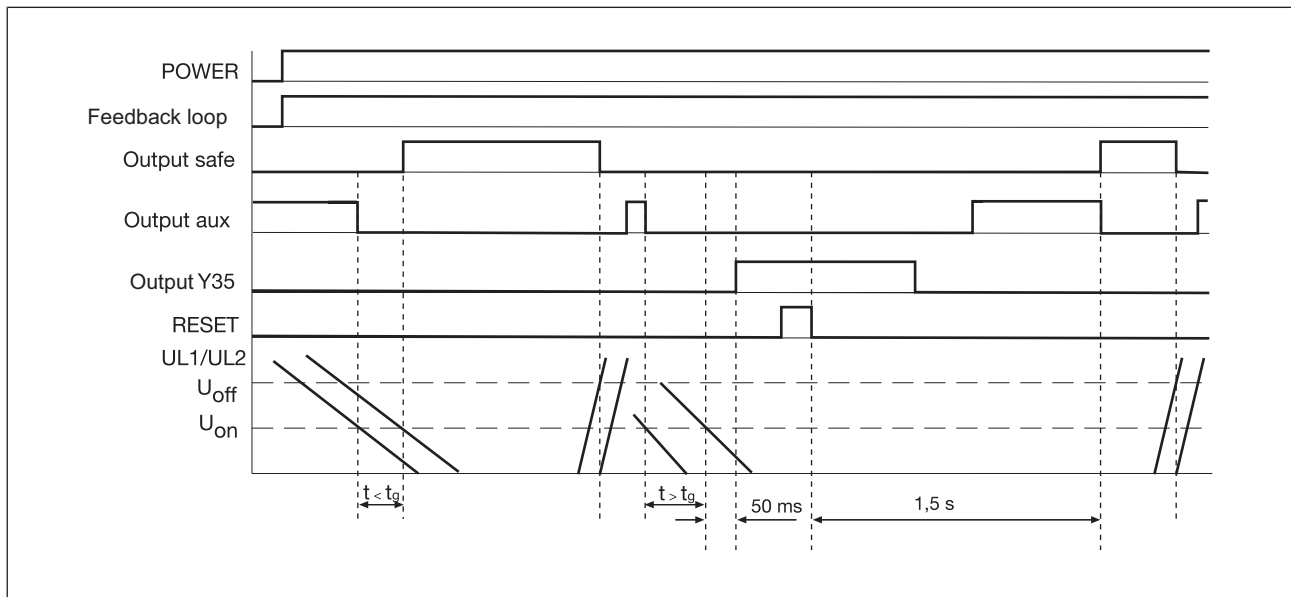
Timing diagram
