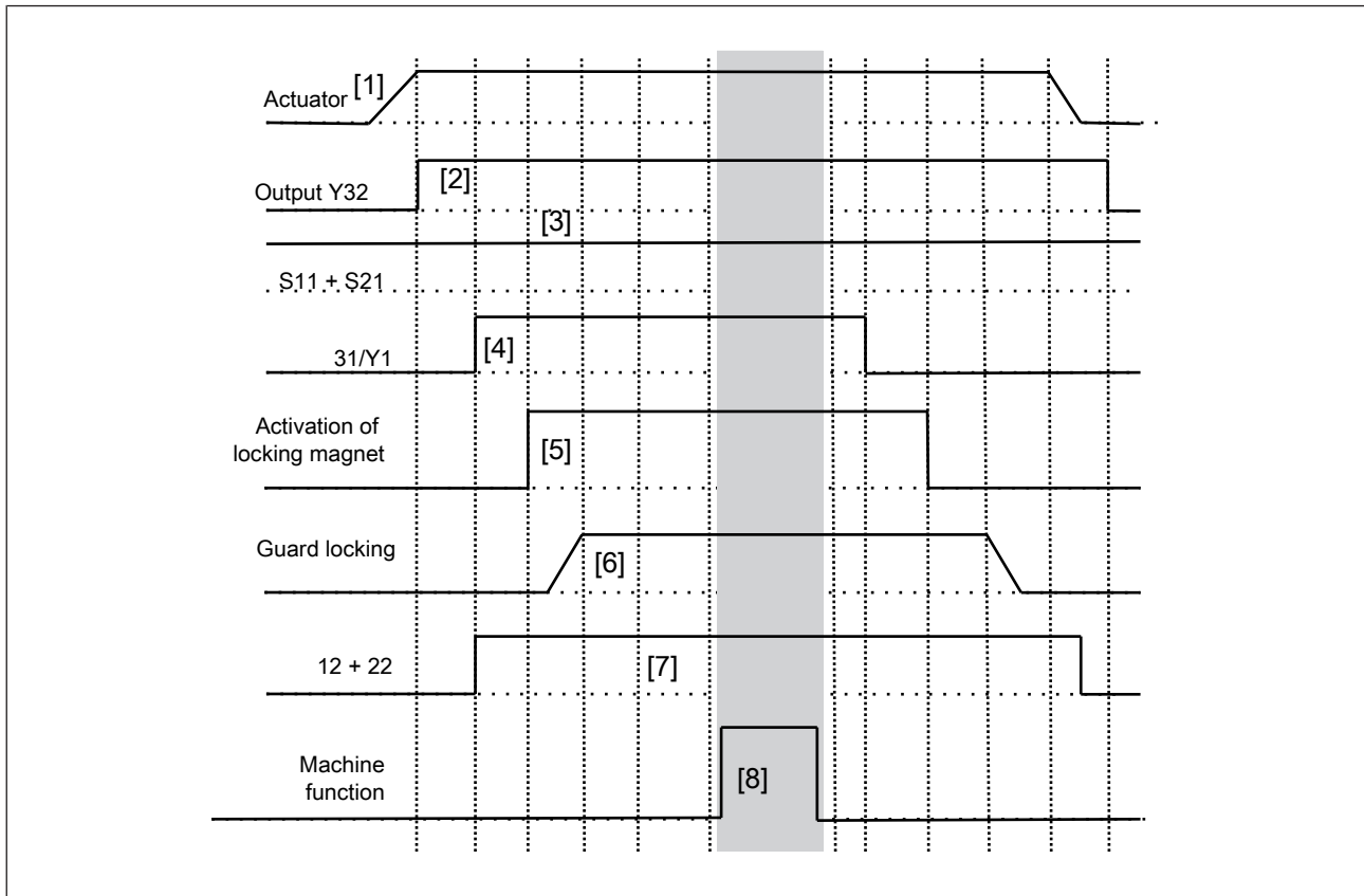
Fig.: Guard locking is controlled via 31
