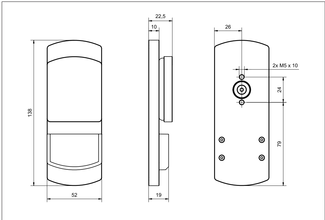
Fig.: Actuator PSEN sl2-1.0 VA actuator - front view, side view, rear view
