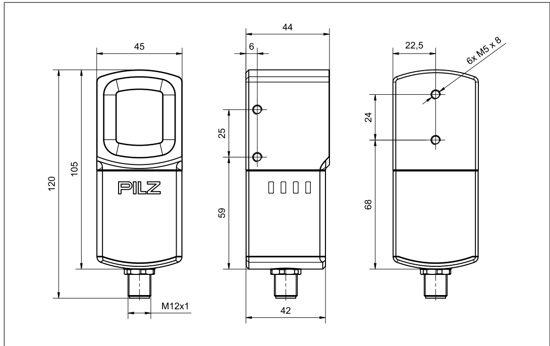
Fig.: Safety switch - front view, side view, rear view
