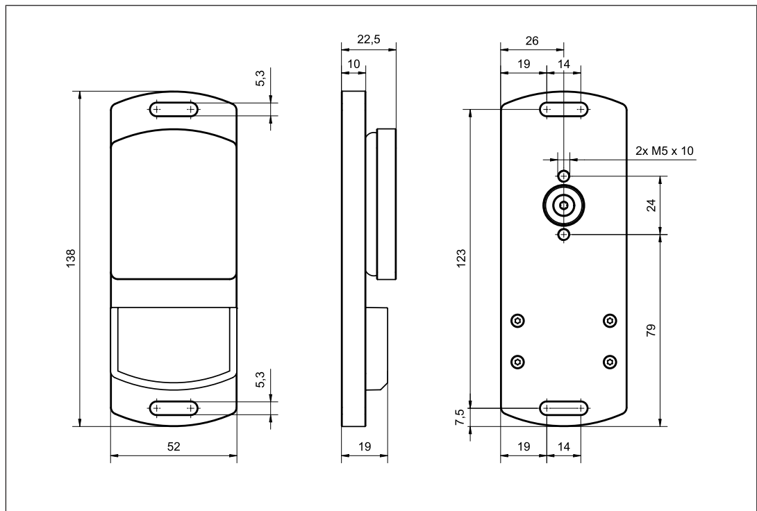
Fig.: Actuator - front view, side view, rear view
