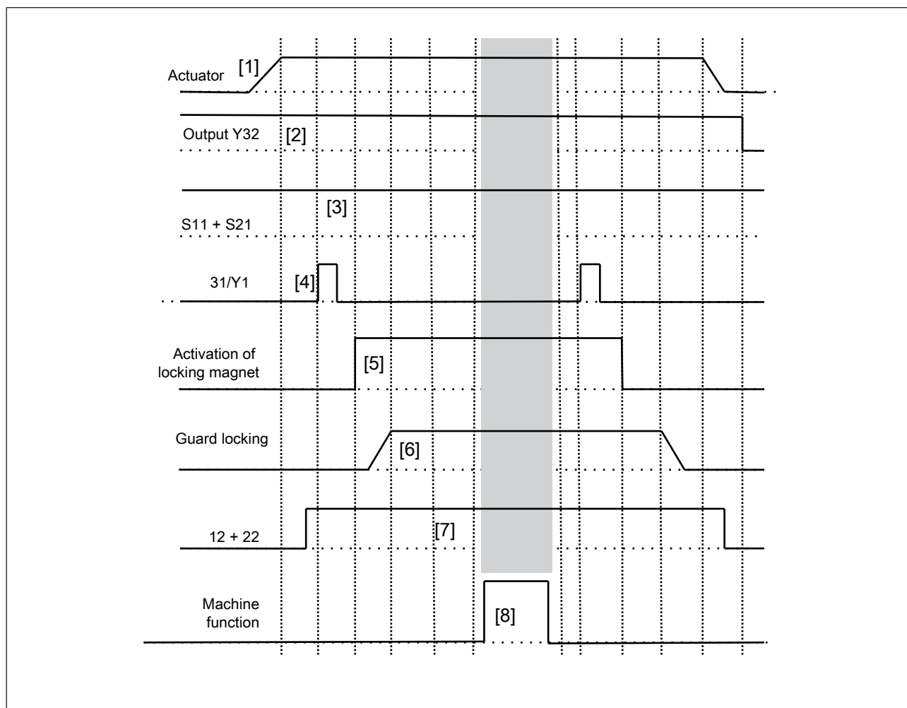
Fig.: Active use of Safety Device Diagnostics
