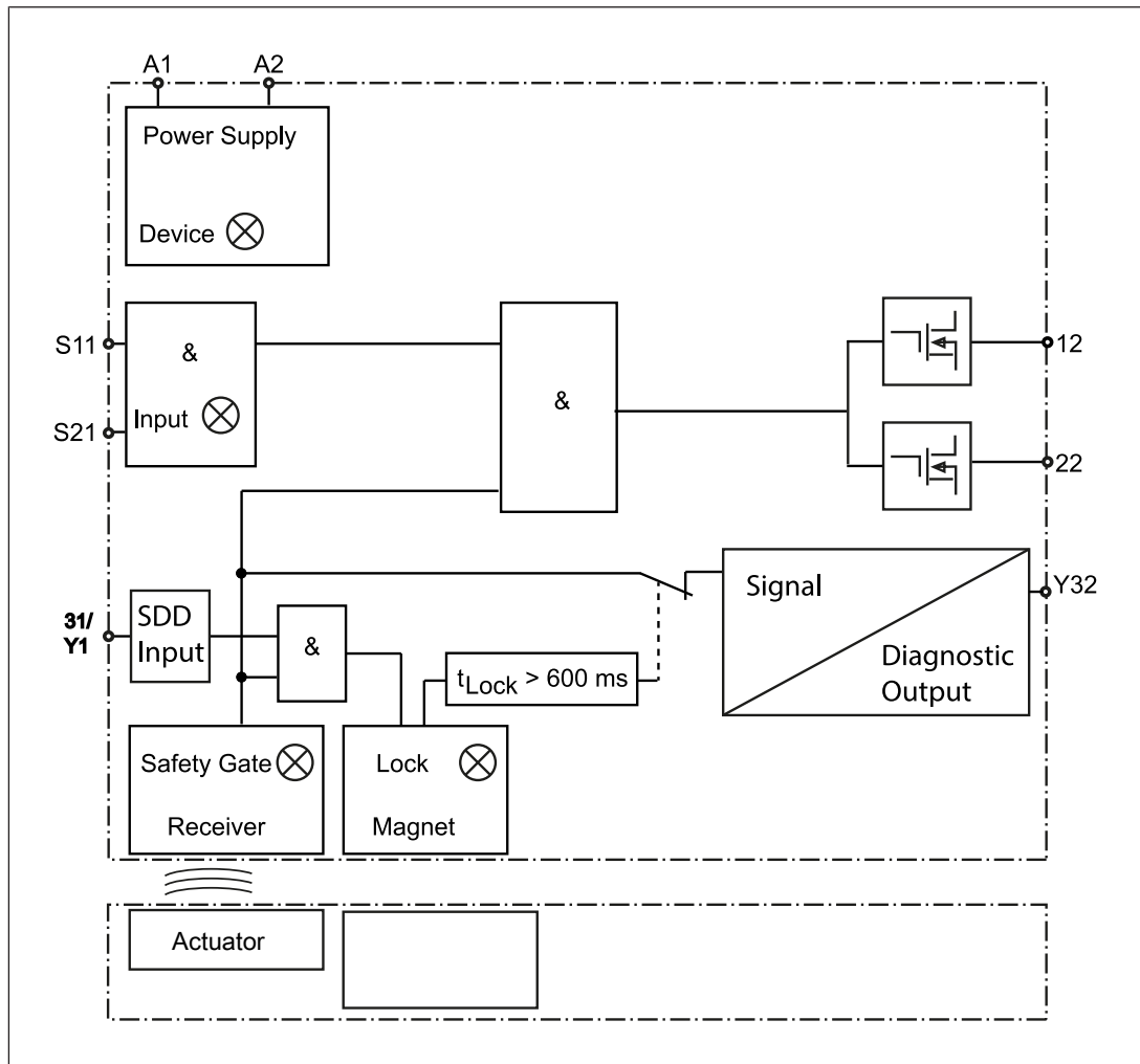
Block diagram
