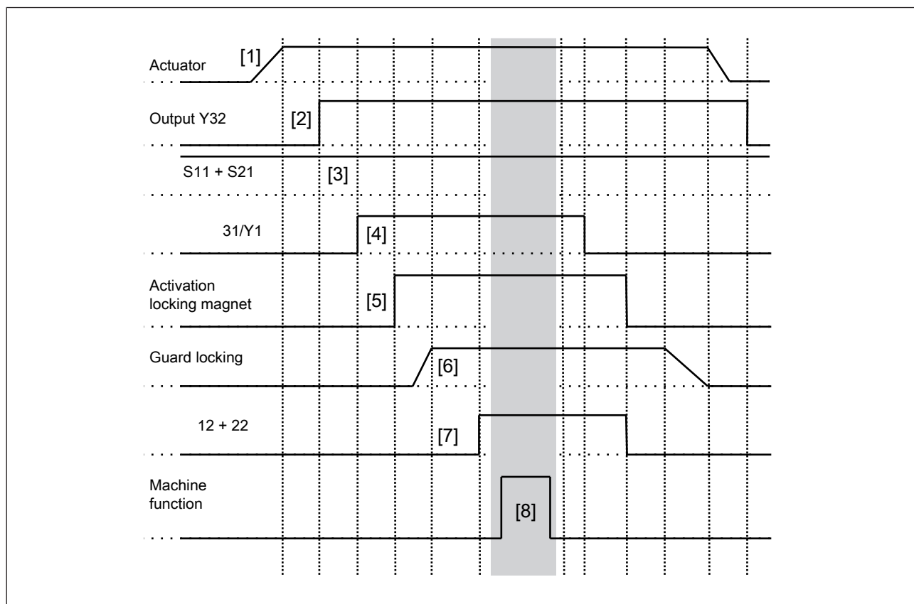
Fig.: Guard locking is controlled via 31/Y1
