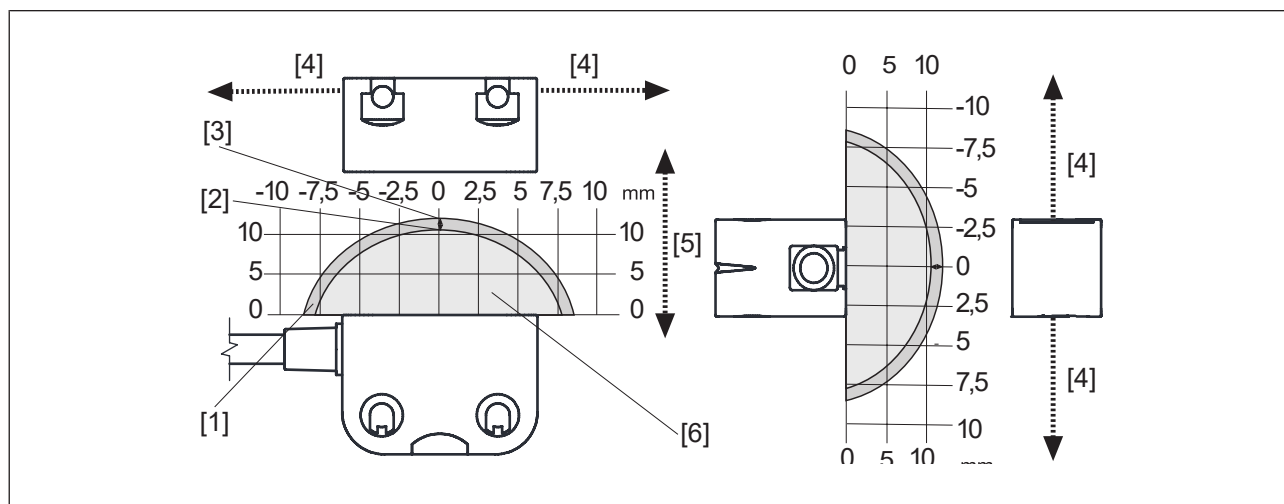
Fig.: Safety switch PSEN cs4.2p/M12 with actuator
