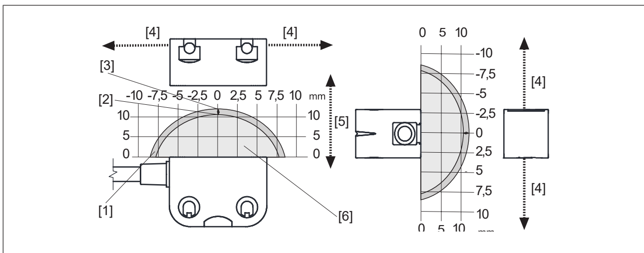
Fig.: Safety switch PSEN cs4.1n with actuator
