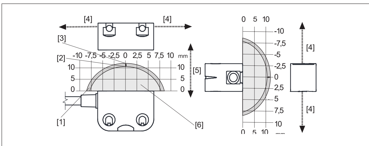
Fig.: Safety switch PSEN cs3.1n with actuator
