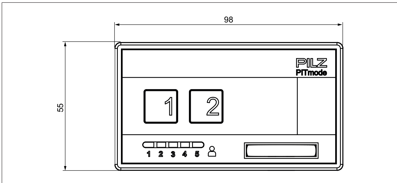
Front view
