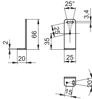
Mounting bracket-11706873
