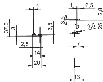
Mounting bracket-11706874
