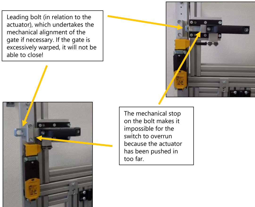
Figure 2: Positioning of bolt
