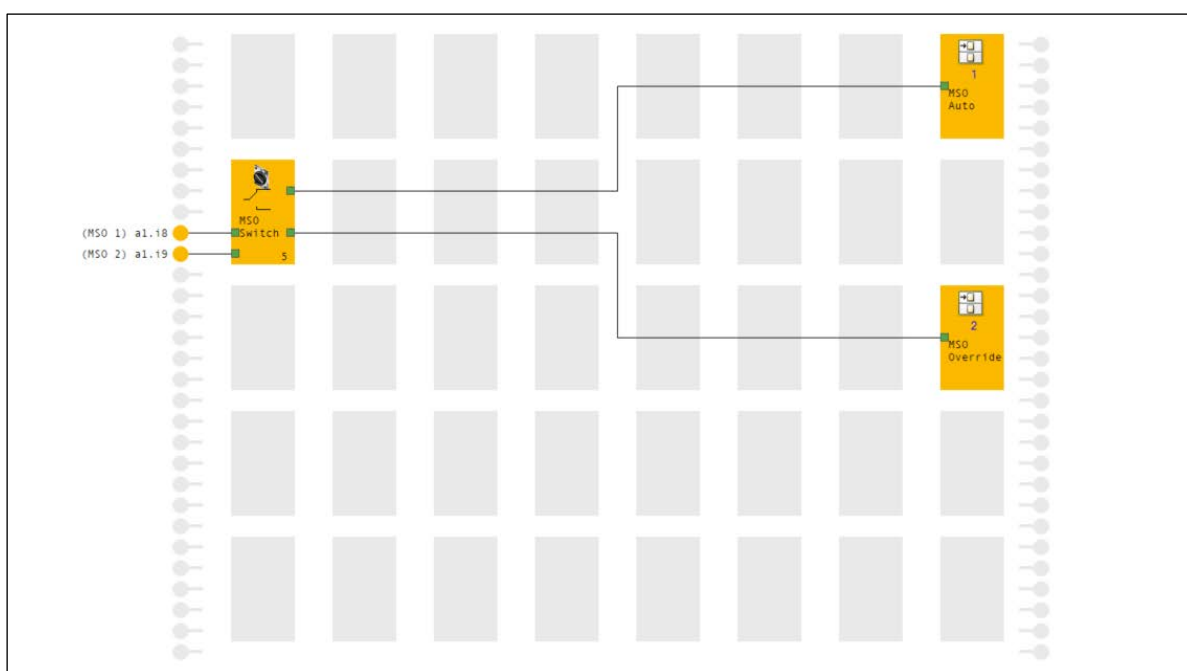
Figure 11: PNOZmulti Configurator – Program, Page 3 » Operating mode selection
