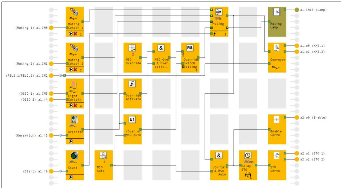
Figure 9: PNOZmulti Configurator – Program, Page 1 » Logic
