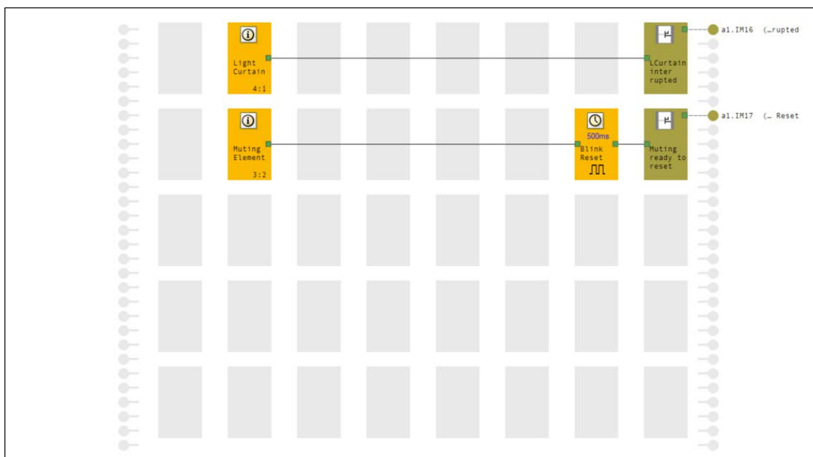
Figure 10: PNOZmulti Configurator – Program, Page 2 » Diagnostics
