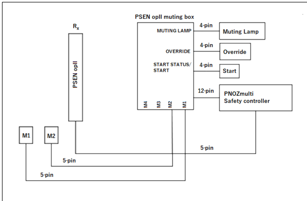
Figure 7: Application – Wiring with the PSEN opII muting box (schematic)
