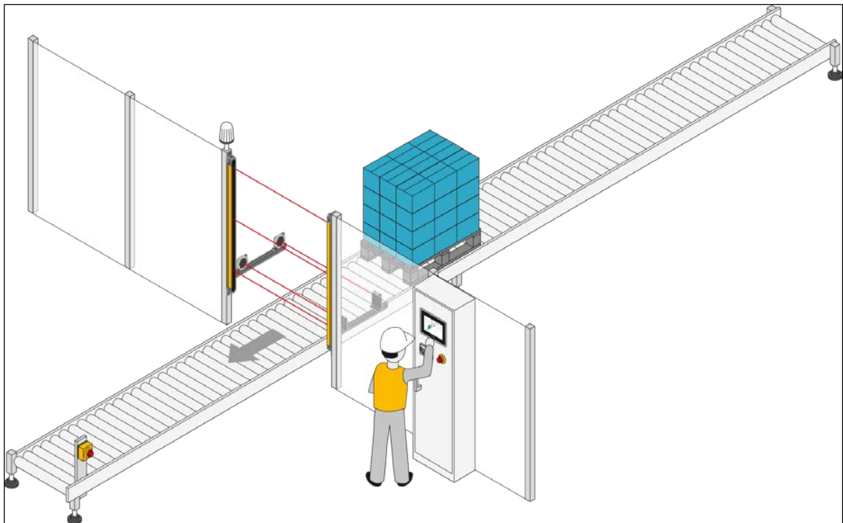
Figure 4: Application – L-muting function (schematic)
