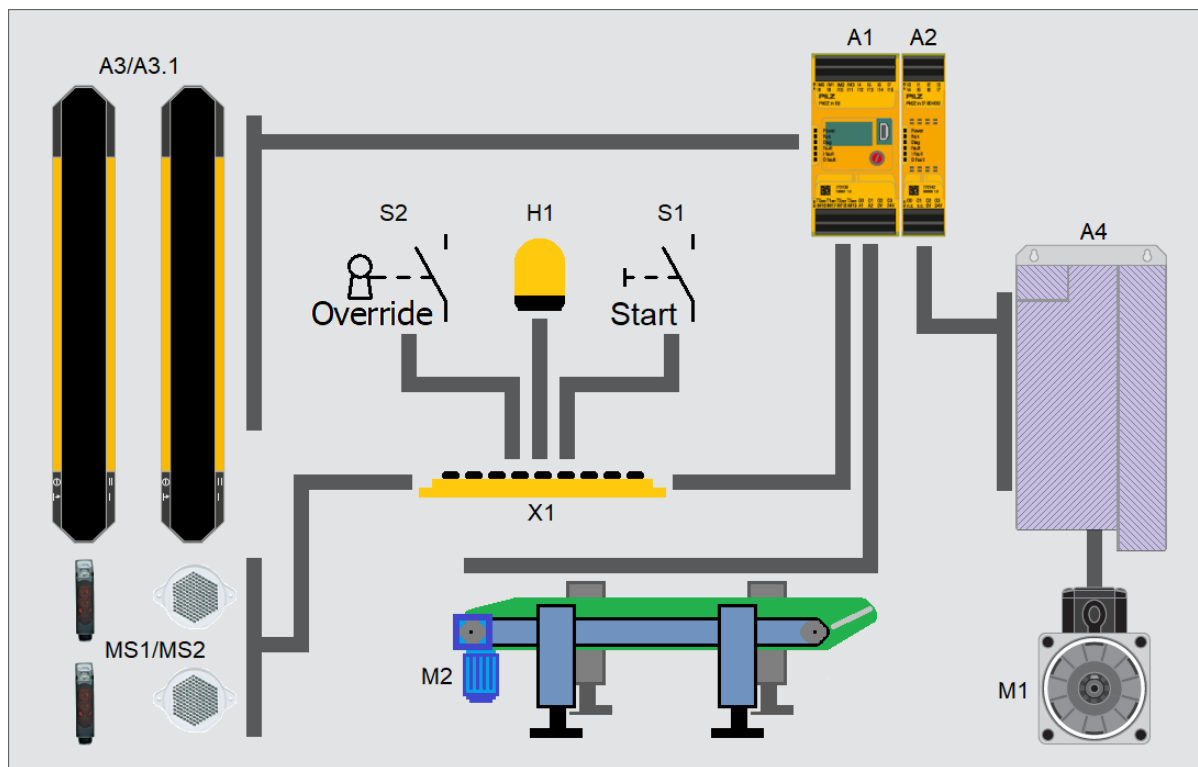
Figure 1: Application – Structure of the hardware (schematic)
